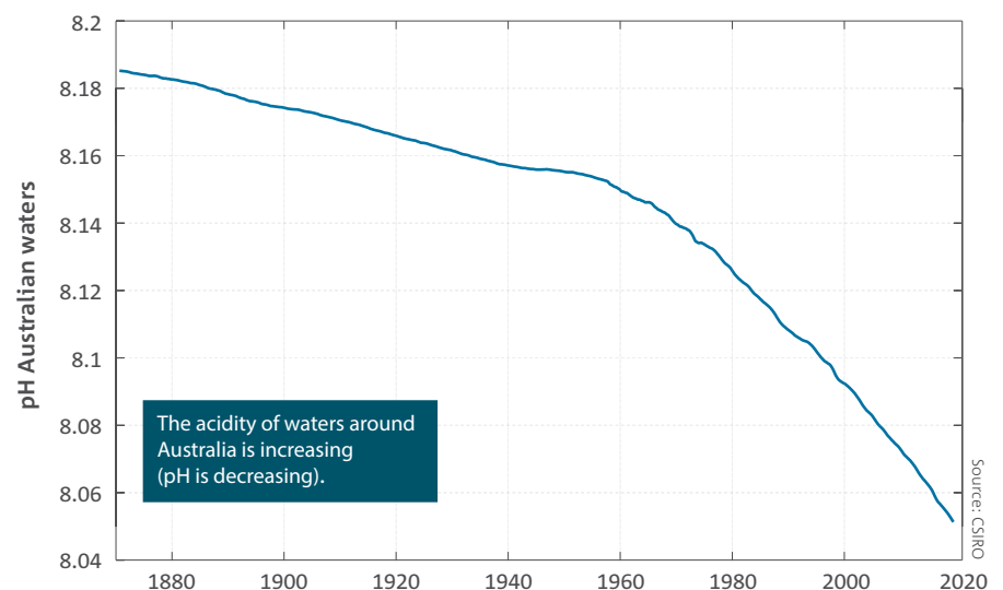
The pH of surface waters around Australia. Top: change between 1880–1889 and 2010–2019, and bottom: the average pH of water surrounding Australia. Calculations are based on present-day data on the carbonate chemistry of surface seawater around Australia from the Integrated Marine Observing System and other programs, and extrapolation of atmospheric carbon dioxide concentration changes since the 1880s.
