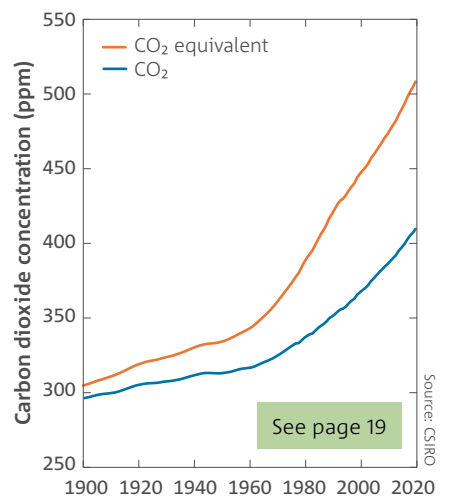
Global mean CO 2 concentration and global mean of all greenhouse gas concentrations expressed as CO 2 equivalent.
