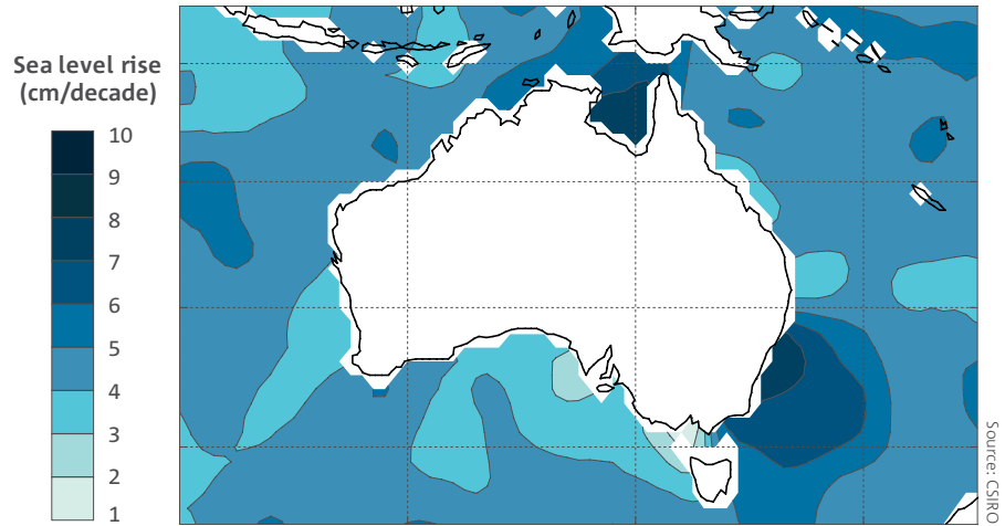
The rate of sea level rise around Australia measured using satellite altimetry, from 1993 to 2019.
