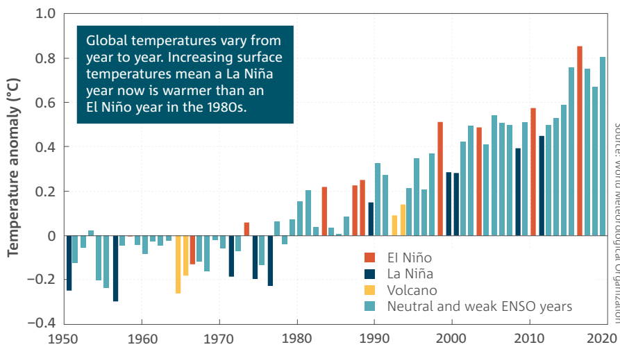
Global surface temperature anomalies of the Earth (land and ocean) for 1950 to 2019. Anomalies are with respect to the 1961–1990 standard averaging period. Major tropical volcanic eruptions are associated with cooler global temperatures. Strong El Niño–Southern Oscillation (ENSO) years see a response in annual global temperatures, such that the year following the start year of an ENSO event is typically warmer than usual with an El Niño, and cooler with a La Niña. This is seen in 2016—the warmest year in this dataset—which followed the start year of the 2015–16 El Niño. Neutral years are those with no moderate or strong El Niño or La Niña events. Data from World Meteorological Organization.
