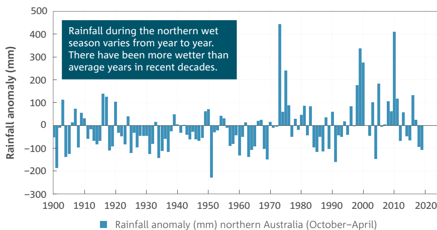
Anomalies of October to April rainfall for northern Australia (north of 26° S inclusive). Anomalies are calculated with respect to the 1961 to 1990 average.
