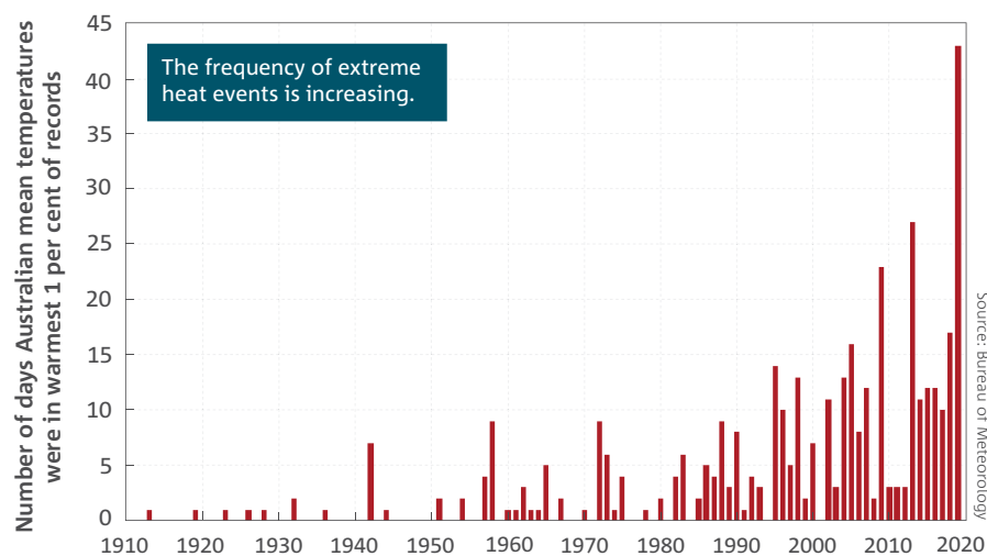
Number of days each year where the Australian area-averaged daily mean temperature for each month is extreme. Extreme daily mean temperatures are the warmest 1 per cent of days for each month, calculated for the period from 1910 to 2019.
