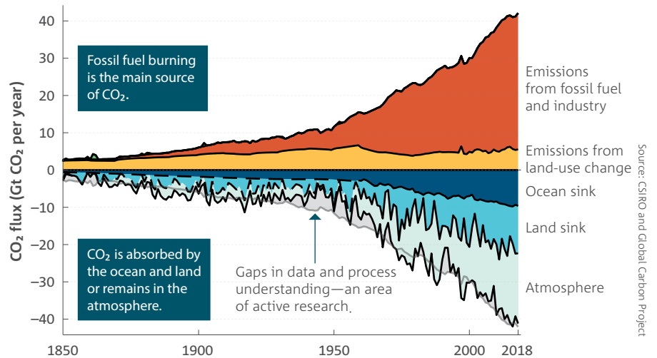
Time series showing the input CO 2 fluxes per year (above zero on plot) from 1850 to 2018 due to emissions from fossil fuels and industry and land-use change; the amount of CO 2 taken up each year by the oceans and land; and the net CO 2 being added each year to the atmosphere.
