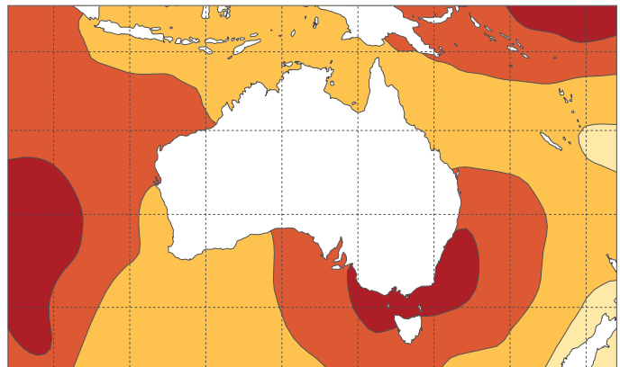
Trends in sea surface temperatures in the Australian region (4–46° S and 94–174° E) from 1950 to 2019.
