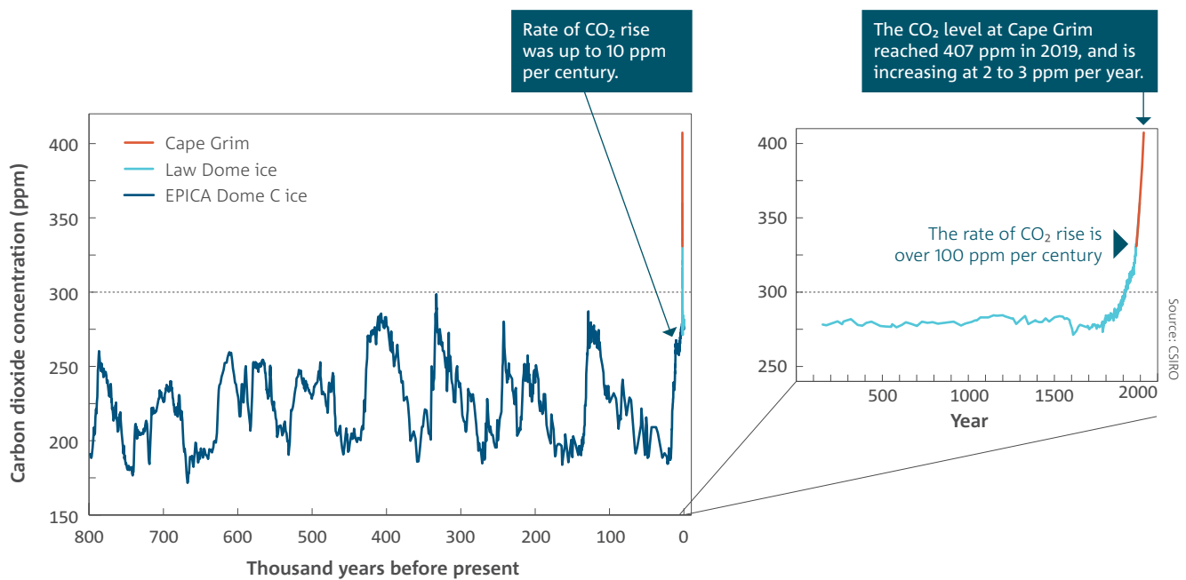
Atmospheric CO 2 concentrations, for the past 800,000 years (left), and for the past 2000 years (right). The time series, and information in the text boxes, are from measurements of air in Antarctic ice cores and at Cape Grim. Though there has been variability in the past, the rate of growth of CO 2 over the past century far exceeds (by a factor of 10 or more) the rate during the most rapid natural changes in the past (which occurred during de-glaciations).
