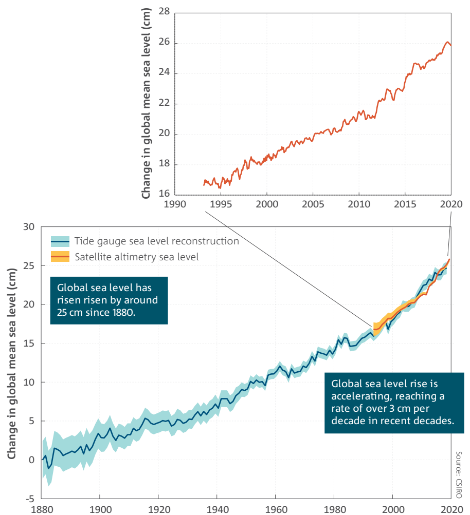
Annual global sea level change from 1880 in tide gauge data (1880–2019, blue line, shading indicates confidence range), and annual sea level change in satellite altimetry (1993–2019, orange line). The pull-out figure shows monthly sea level change from 1993 to 2019, measured using satellite altimetry from 1993 to 2019.
