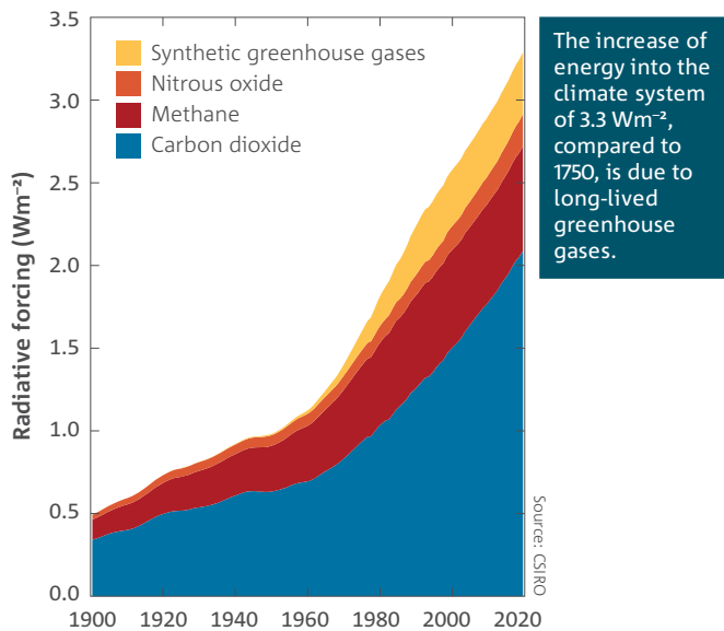
Left: Radiative forcing relative to 1750 due to the long-lived greenhouse gases carbon dioxide, methane, nitrous oxide and the synthetic greenhouse gases, expressed as watts per metre squared. Right: Global mean CO 2 concentration and global mean greenhouse gas concentrations expressed as CO 2 equivalent (ppm). CO 2 equivalent is calculated from the atmospheric concentrations of carbon dioxide, methane, nitrous oxide and the suite of synthetic greenhouse gases.
