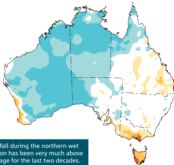
Northern wet season (October–April) rainfall deciles for the last 20 years (2000–01 to 2019–20). A decile map shows where rainfall is above average, average or below average for the recent period, in comparison with the entire national rainfall record from 1900.
