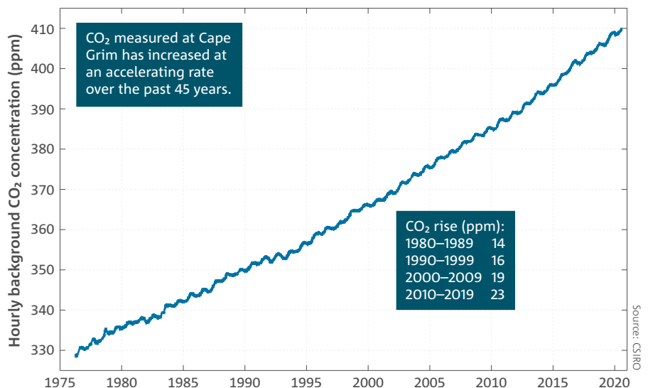
Background hourly clean-air CO 2 as measured at the Cape Grim Baseline Air Pollution Station from 1976 through to June 2020. The hourly data represent thousands of individual measurements. To obtain clean air measurements, the data are filtered to include only periods when air has come across the Southern Ocean and is thus free from local sources of pollution. The increase in CO 2 concentration for each decade from 1980 to 2019 (1 January for the start year and 31 December for the end year) is also shown.
