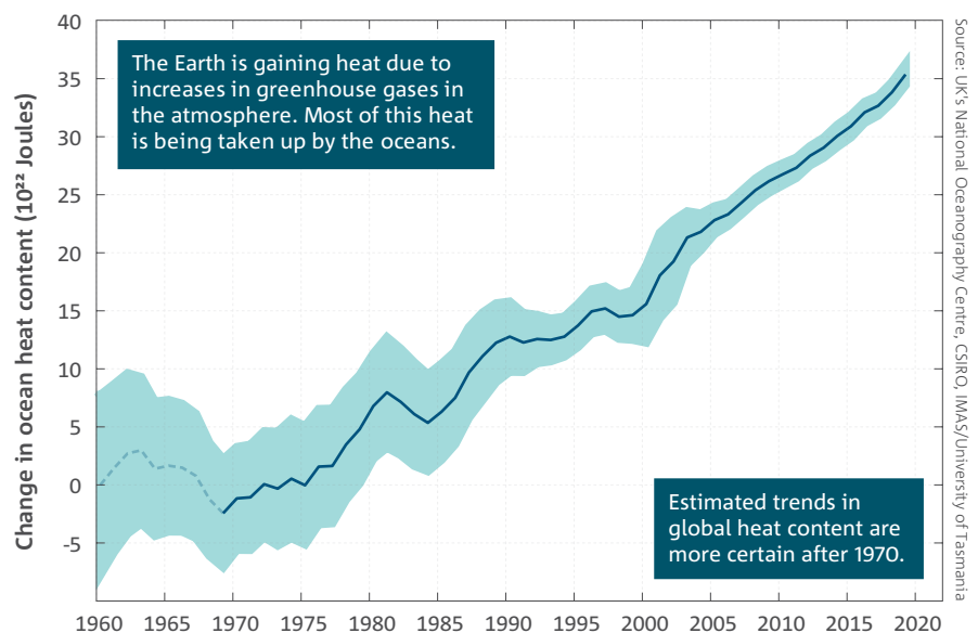
Estimated change in ocean heat content over the full ocean depth, from 1960 to 2019. Shading provides an indication of the confidence range of the estimates. The measurements contributing to the early part of the record, before 1970, are sparse and trends estimated over this period are small compared to the confidence range and hence are considered less reliable.
