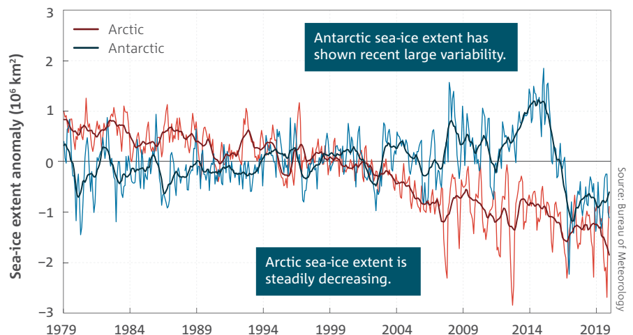
Antarctic and Arctic sea-ice extent (shown as the net anomaly from the 1981–2010 monthly averages in order to remove the seasonal variability) for the period January 1979 to December 2019 (10 6 km 2 ). Thin lines are monthly averages and indicate the variability at shorter time-scales, and thick lines are eleven-month running averages.
