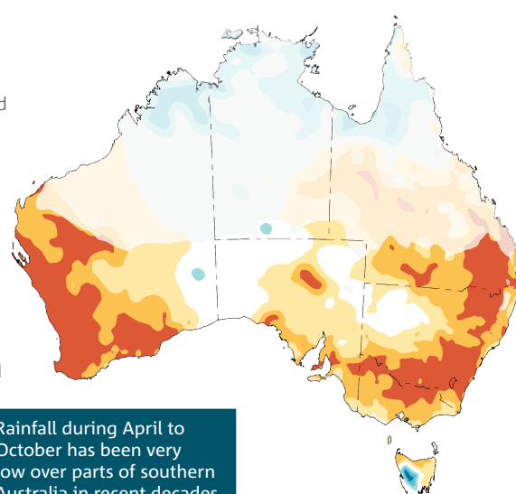
April to October rainfall deciles for the last 20 years (2000–19). A decile map shows where rainfall is above average, average or below average for the recent period, in comparison with the entire rainfall record from 1900. Areas across northern and central Australia that receive less than 40 per cent of their annual rainfall during April to October are faded.
