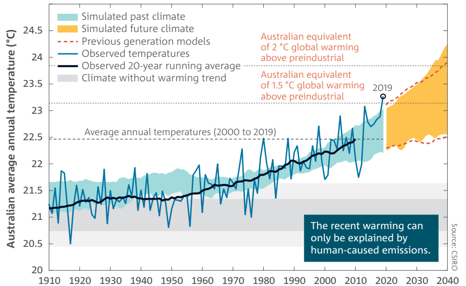
Australian average annual temperature observed and simulated from global climate models. Past and future bands show the range of 20-year running average of new generation climate model results, dashed lines show the equivalent from the previous generation of global climate models. Climate without warming trend shows both an inner and an outer band which are one and two standard deviations, respectively, from the 1850–1900 average, i.e. prior to the rapid growth in greenhouse gas emissions from human activities. The black dashed lines show the Australian equivalent of the global warming thresholds 1.5 °C and 2 °C above the pre-industrial baseline period 1850–1900, equating to warming levels of around +2.1 °C and +2.8 °C respectively, based on the observed ratio of Australian to global temperature of around 1.4.
