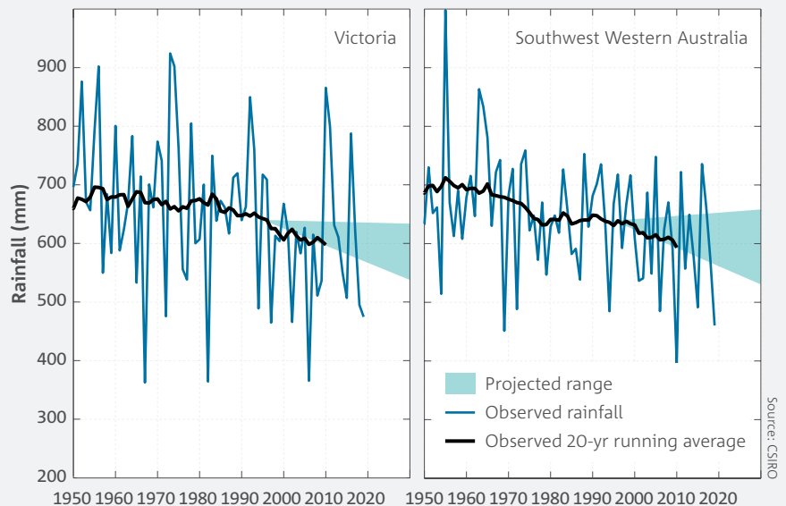
Evaluation of average annual rainfall projections for two example regions in Australia. Projected range starts at 1995 (mid-point of the 1986–2005 baseline). Left: For Victoria, projection from the Victorian Climate Projections 2019 VCP19; Right: Southwest Western Australia, projection from Climate Change in Australia, the national climate change projections for Australia. Southwest Western Australia is defined as a cluster of Natural Resource Management regions covering the southwest of the State; and differs from the area in the rainfall section.
