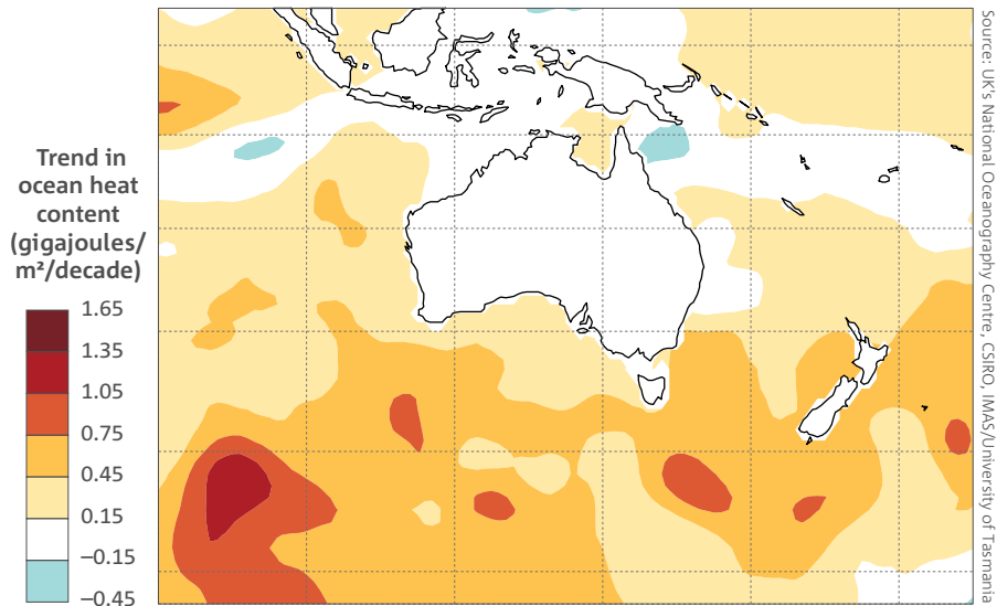
Estimated linear decadal trend in ocean heat content between 1970 and 2019 in the upper 2000 m of the ocean, showing the highest uptake of heat in regions where the circulation draws heat into the deep ocean, such as the Southern Ocean.
