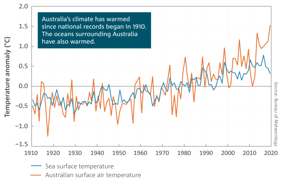
Anomalies in annual mean sea surface temperature, and temperature over land, in the Australian region. Anomalies are the departures from the 1961–1990 standard averaging period. Sea surface temperature values (data source: ERSST v5, www.esrl.noaa.gov/psd/ ) are provided for a region around Australia (4–46 °S and 94–174 °E).
